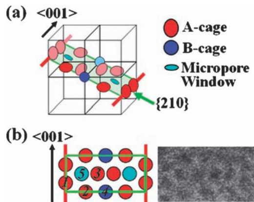
Figure 3. (a) The schematic pore arrangement on the \{210\} plane of SBA-1 expected from Ref 13. (b) The actual pore arrangement of the \{210\} plane and FESEM image of the outermost surface. The pore arrangement of the outermost surface is represented by five nonequivalent pores (Nos. 1–5).
