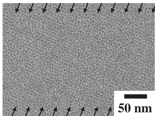
Figure 1. FESEM image of the typical outermost surface of calcined MPS film. The location of “straight lines” is shown by arrows.
